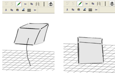
(c) Object anchoring by drawing a line between the ground and object. The line also indicates which face of the object touches the ground.
