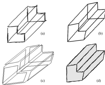
Figure 4: 3D reconstruction pipeline: (a) the input rough sketch, (b) the cleaned 2D graph, (c) the recognized faces, and (d) the recognized object.
