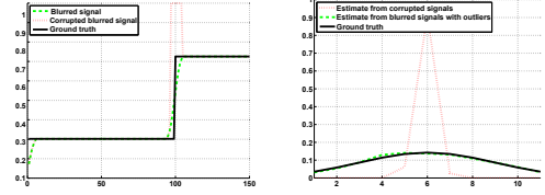
Figure 6. Effects of outliers on kernel estimation. (b) shows the results of [36] using the signals shown in (a).
