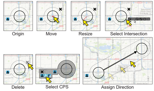
Figure 7: Trajectory Filtering Interactions. CPS is short for Carry Passenger Status.
