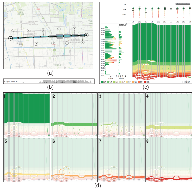
Figure 10: TrajRank with Even Segmentation: (a) a westward route is selected on the 4th ring; (b) the horizon graph shows the temporal distribution of trajectories on that route; (c) ranking diagram shows the trajectory ranking; (d) 8 clusters with different travel behaviors are highlighted respectively.
