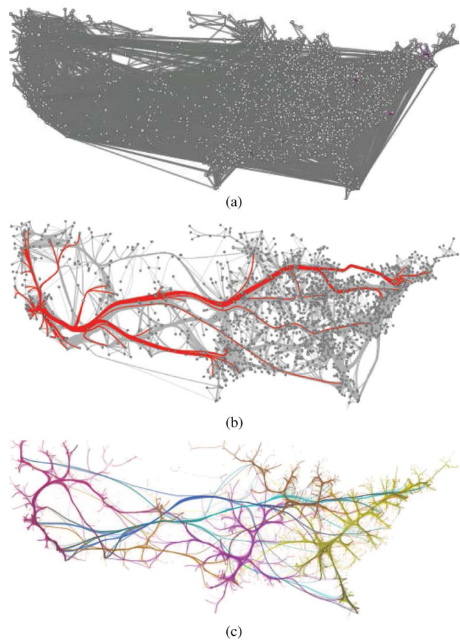
Fig. 8. (a) Line-based visualization of the immigration information in the USA [79]; (b) edge bundling result generated by [80]; (c) edge bundling result generated by [81].
