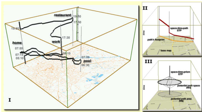
Fig. 12. Space-time-cube: both spatial information and temporal information are visualized in a cube [84]. The X-axis and Y-axis represent spatial information, whereas the Z-axis represents temporal information.
