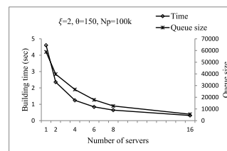
Fig. 9. Scalability of DSI w.r.t. the number of servers.
