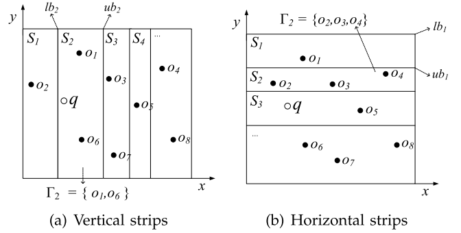
Fig. 1. The elements of the DSI index structure.
