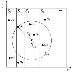
Fig. 4. An example of finding three-NN using DKNN.
