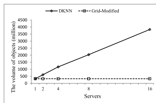
Fig. 14. The largest datasets supported by DKNN and Grid-Modified.
