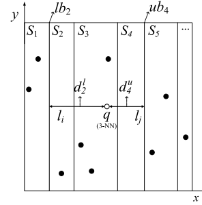
Fig. 3. Determining the set of candidate strips.
