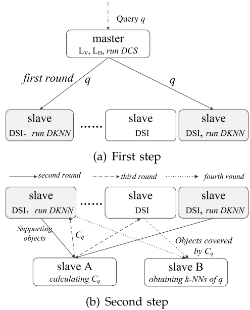
Fig. 5. Processing queries on the master-slaves model.
