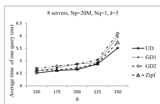
Fig. 19. Performance of DKNN w.r.t. \theta .
