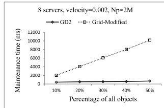
Fig. 13. Comparison of DKNN and Grid-Modified w.r.t maintenance cost.
