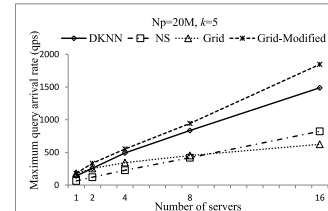
Fig. 16. Throughput of DKNN.
