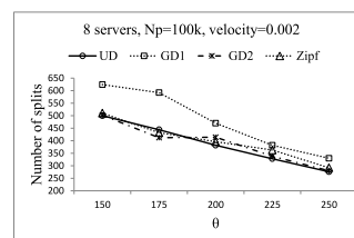
Fig. 10. Number of splits w.r.t \theta .
