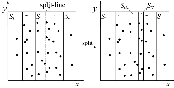
Fig. 2. The split of S_i .
