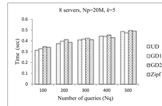
Fig. 15. Performance of DKNN w.r.t number of queries.
