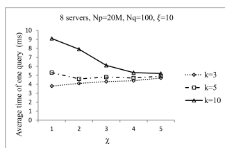
Fig. 18. Performance of DKNN w.r.t. \chi .
