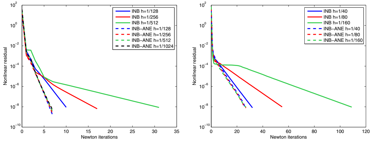
Fig. 6. Convergence histories of INB and INB-ANE for different mesh sizes, the airfoil case, M_\infty = 0.8 (left) and the channel flow case, M_\infty = 0.8435 (right).
