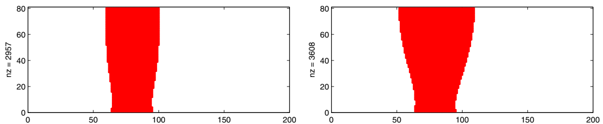
Fig. 8. The channel flow case. The final distribution of the bad components. h = 1/40 with M_\infty = 0.835 (left) and M_\infty = 0.8435 (right), M_c = 0.85 . The red region means the collection of bad components. (For interpretation of the references to color in this figure legend, the reader is referred to the web version of this article.)
