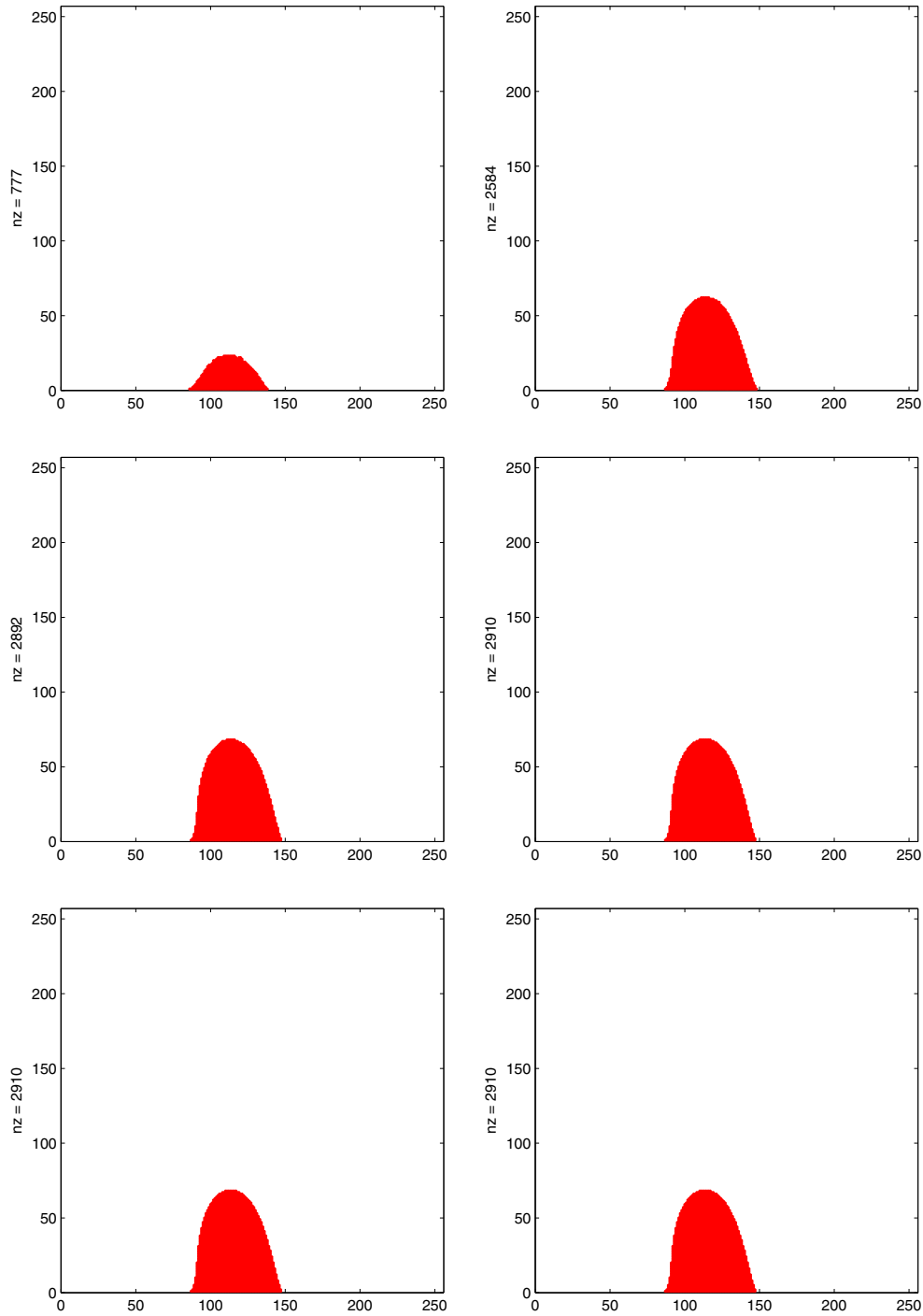
Fig. 7. The airfoil case. The evolution of the distribution of the “bad” components during the global Newton iterations. The red area means the collection of the bad components. Mesh size, h = 1/256 . “nz” is the total number of bad components. (For interpretation of the references to color in this figure legend, the reader is referred to the web version of this article.)
