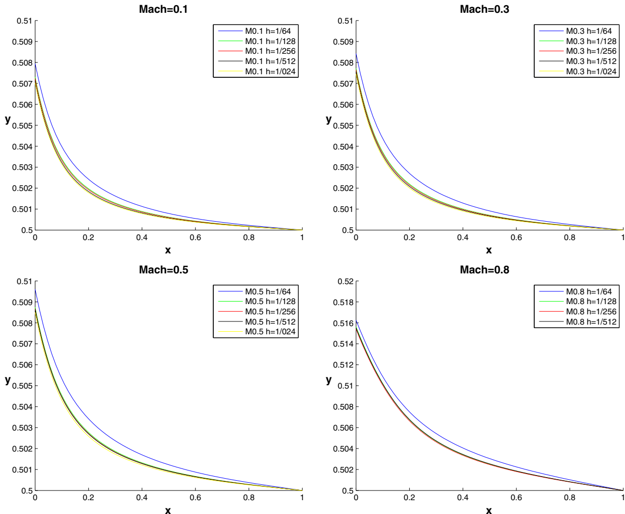
Fig. 2. The airfoil case. Computed potential curves along the vertical midline at x = 0.5 for different values of M_\infty = 0.1 (top-left), 0.3 (top-right), 0.5 (bottom-left), and 0.8 (bottom-right) and different mesh sizes.
