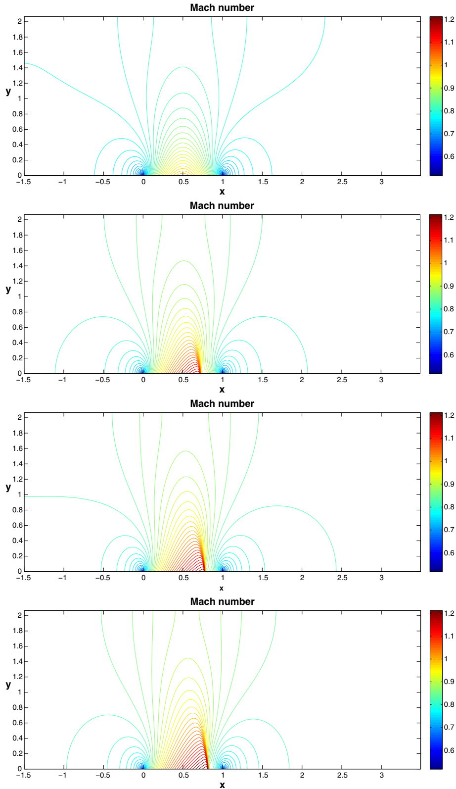
Fig. 4. The channel flow case. The Mach number contours for M_\infty = 0.8, 0.835, 0.8435 , and 0.85 (from top to bottom) obtained by the numerical solution using INB-ANE on a mesh with h = 1/160 .
