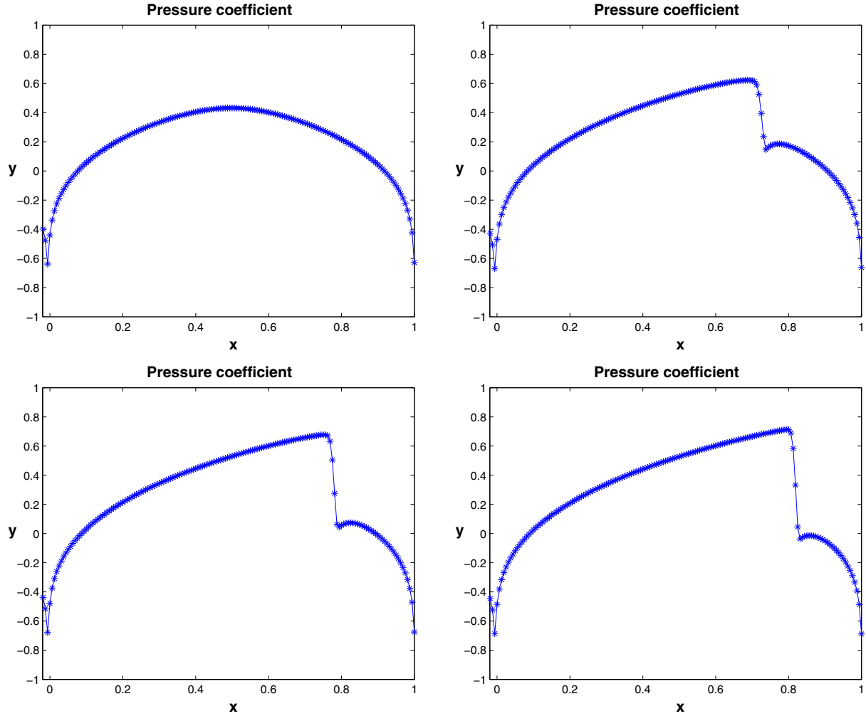
Fig. 5. The channel flow case. The plots of the pressure coefficients for M_\infty = 0.8 (top-left), M_\infty = 0.835 (top-right), M_\infty = 0.8435 (bottom-left), and M_\infty = 0.85 (bottom-right) obtained by the numerical solution using INB-ANE on a mesh with h = 1/160 .
