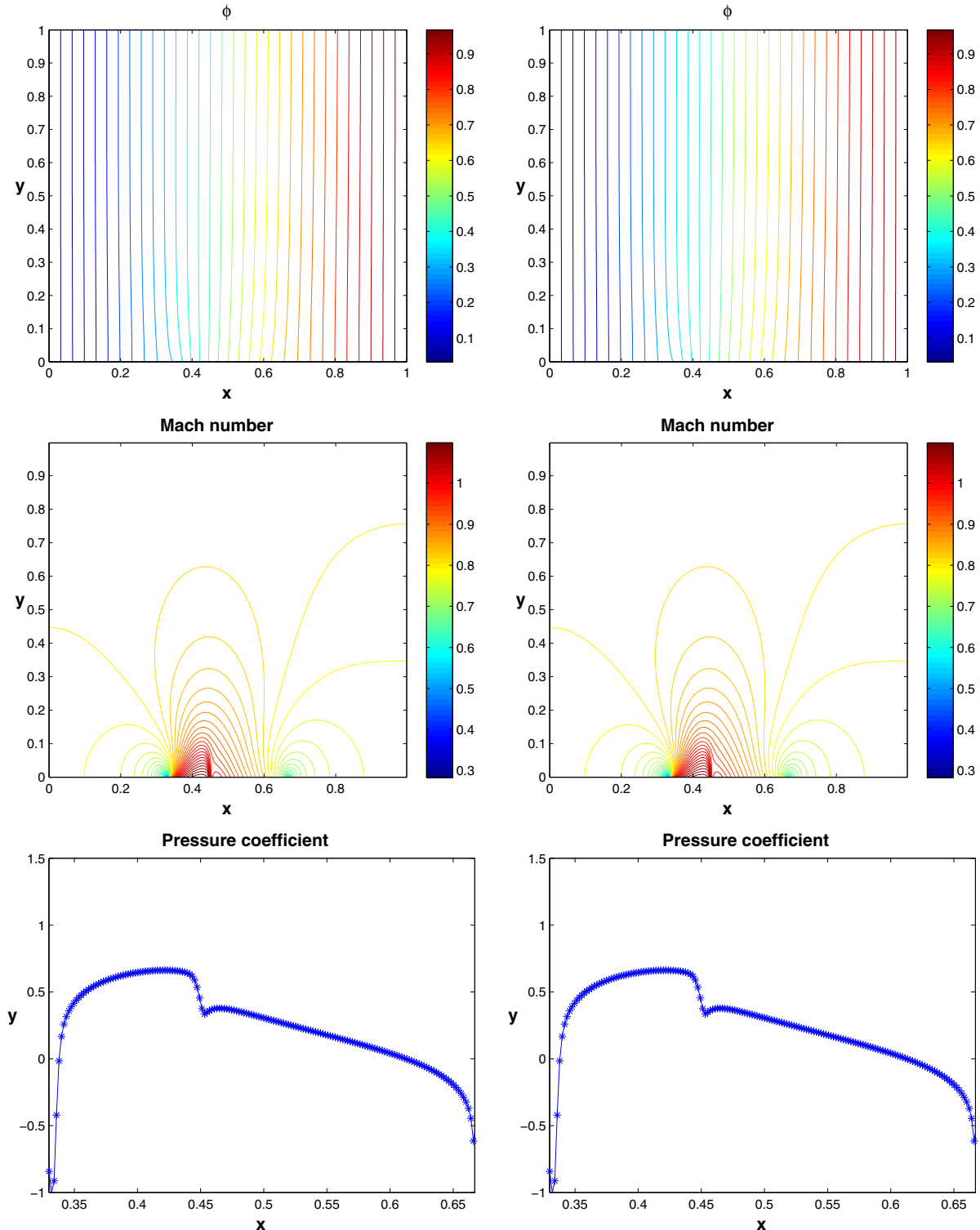
Fig. 3. The airfoil case. A comparison of potential contours (1st row), the Mach number contours (2nd row), and the pressure coefficients (3rd row) obtained by the numerical solution using INB (left column) and INB-ANE (right column). M_\infty = 0.8 and h = 1/512 .
