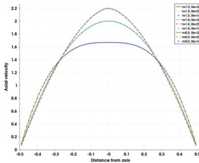
Figure 3. The velocity profile with different n and Re .
