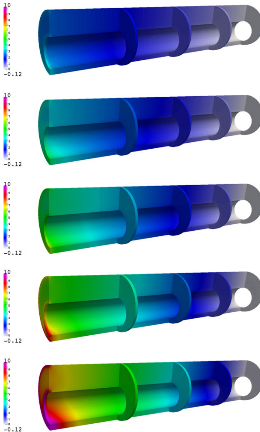
Figure 9. Pressure distributions for the cases with different values of the power-law index in the order of n = 0.50, 0.75, 1.0, 1.25 , and 1.50 .
