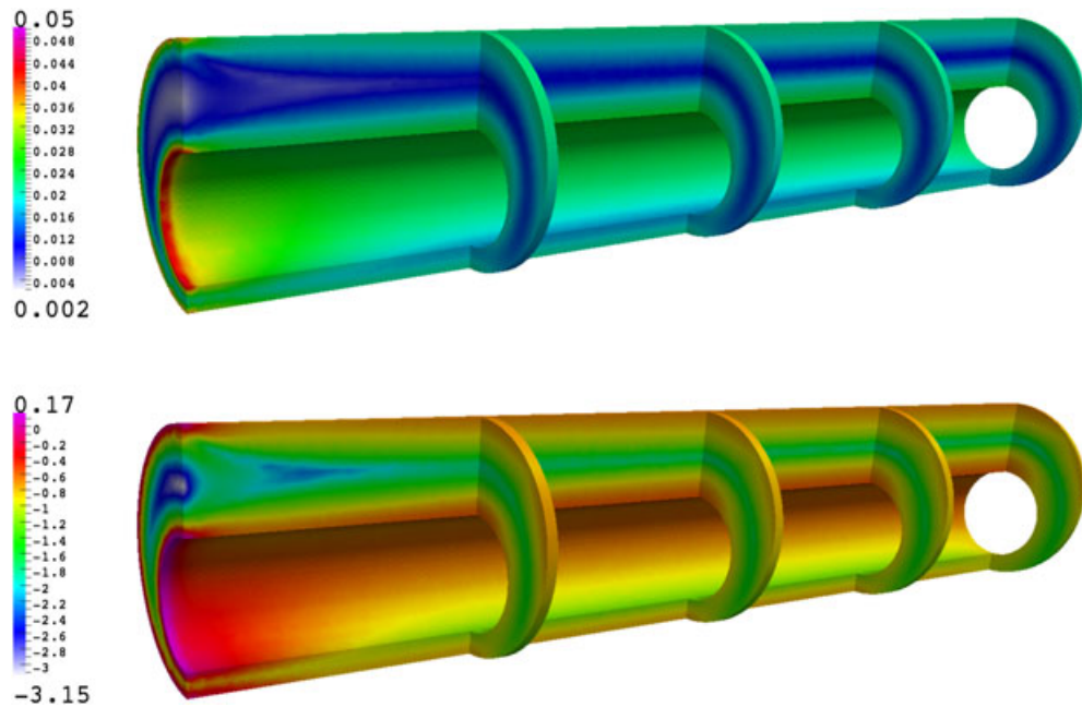
Figure 8. A comparison of viscosity (top) and shear stress in the logarithmic scale (bottom) for the case of dilatant ( n = 1.5 ).
