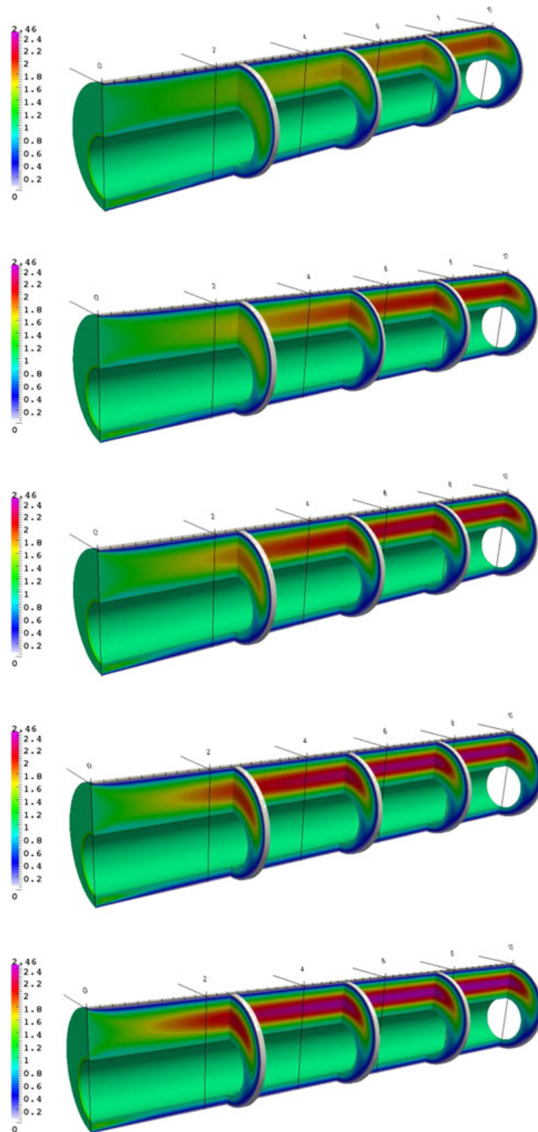
Figure 10. Velocity distributions for the cases with different values of the power-law index in the order of n = 0.50, 0.75, 1.0, 1.25 , and 1.50 .
