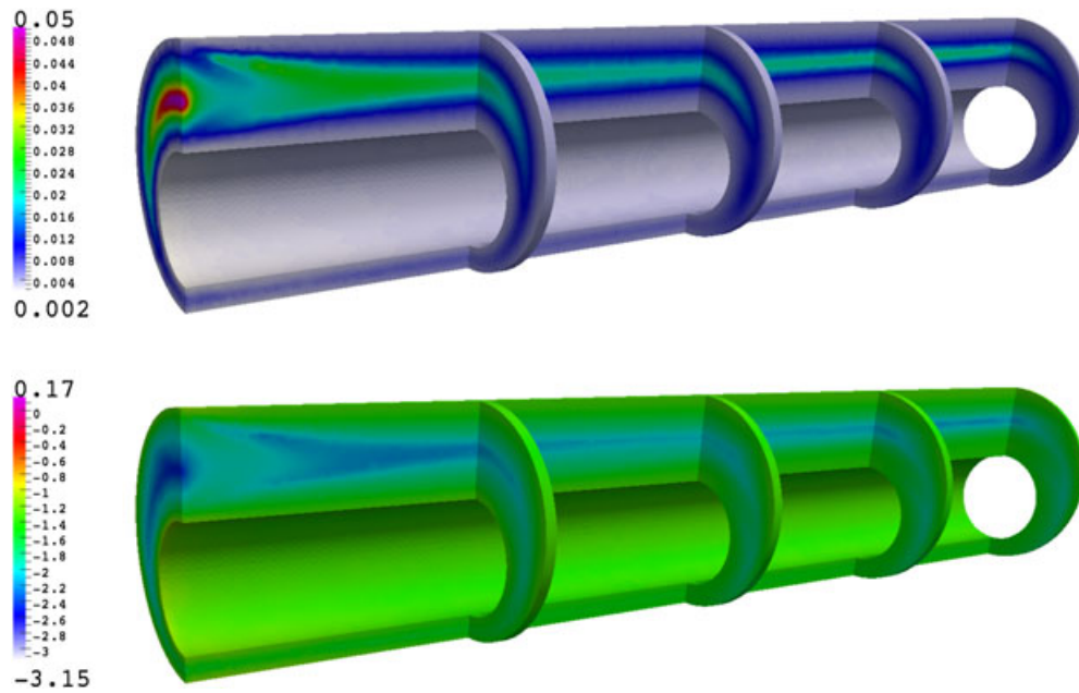
Figure 7. A comparison of viscosity (top) and shear stress in the logarithmic scale (bottom) for the case of pseudoplastic ( n = 0.5 ).
