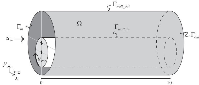
Figure 4. 3D rotational eccentric annulus geometry.
