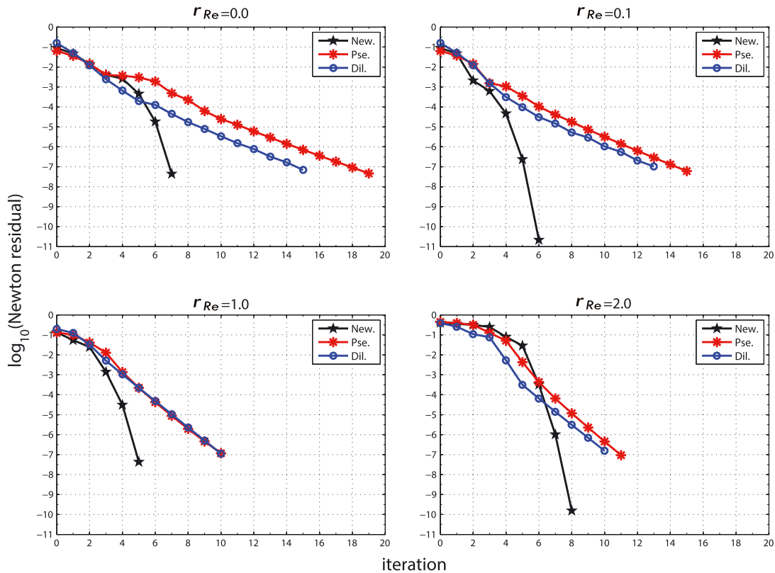
Figure 6. Histories of nonlinear residuals for different r_{Re} . Here, 'New.' is for Newtonian flows, 'Pse.' is for n = 0.75 case, and 'Dil.' is for n = 1.25 case.
