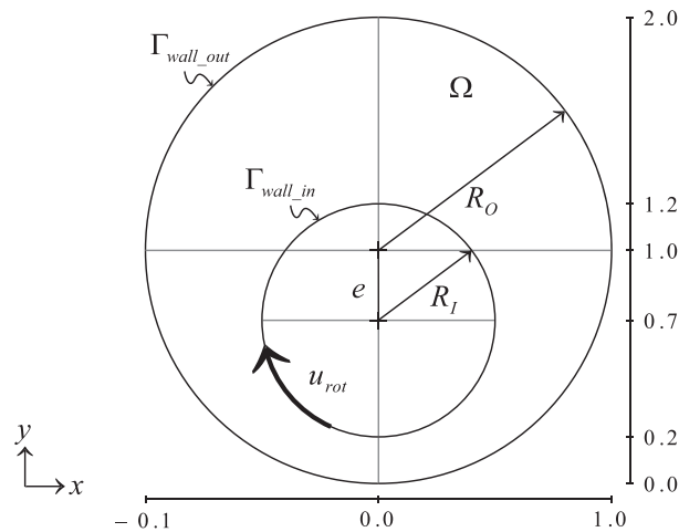
Figure 5. Schematic view of 3D rotational eccentric annulus cross section.
