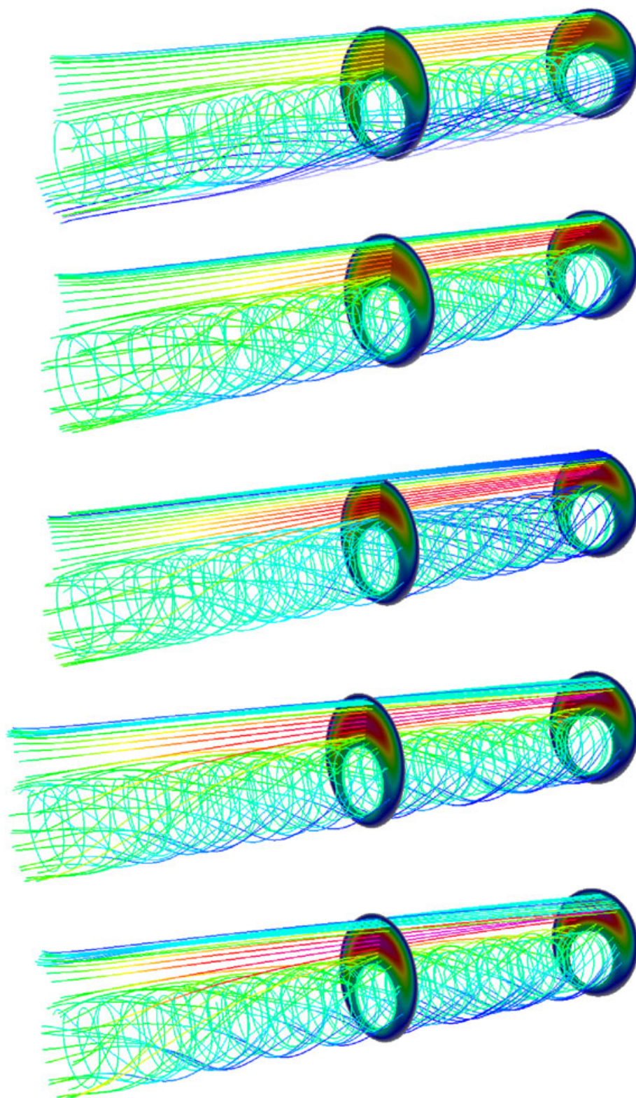
Figure 11. Streamlines for the cases with different values of the power-law index in the order of n = 0.50, 0.75, 1.0, 1.25 , and 1.50 .
